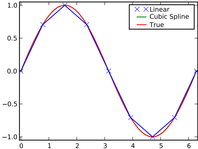
Cubic-spline interpolation
