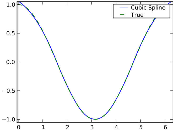
Derivative estimation from spline
