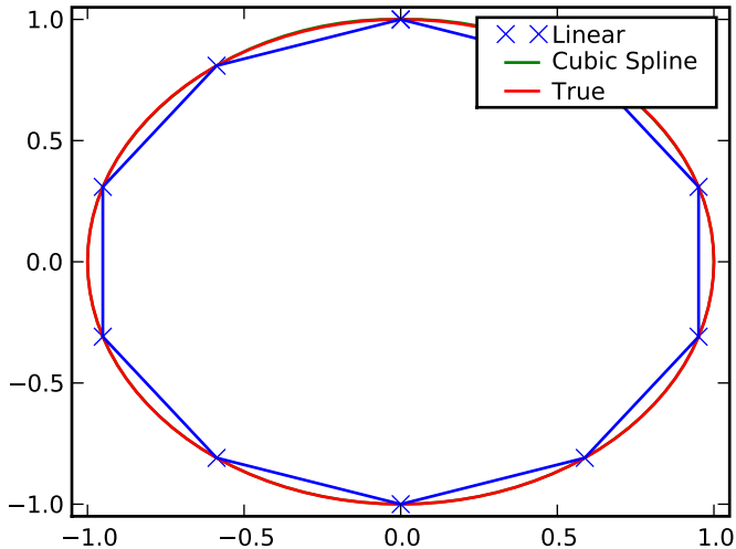
Spline of parametrically-defined curve
