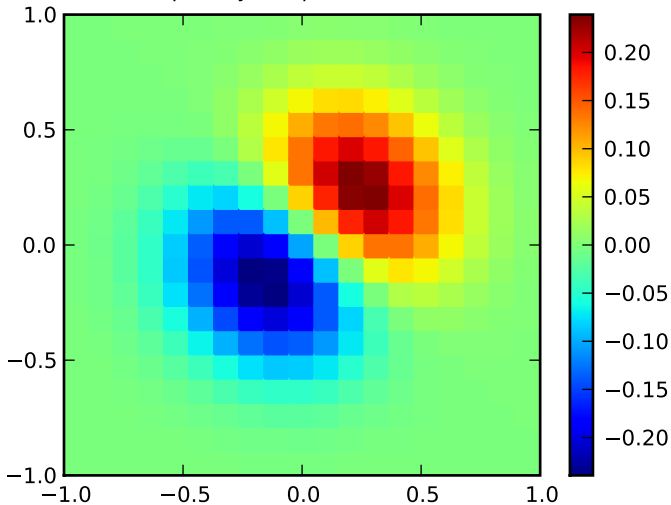
Sparsely sampled function.
